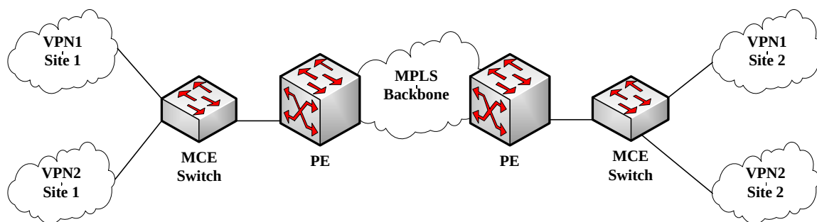
MCE in the MPLS-VRF VPN network
