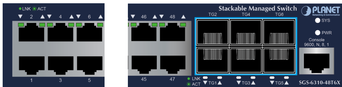
Figure SGS-6310-48T6X front panel
