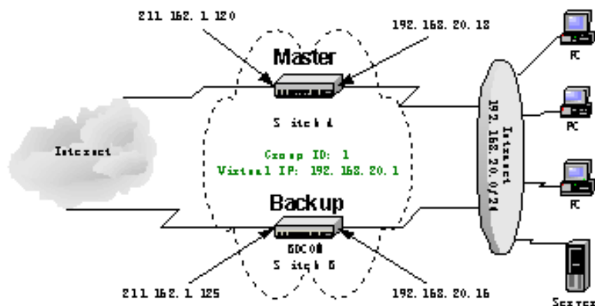
Figure1 69-1 Network topology
