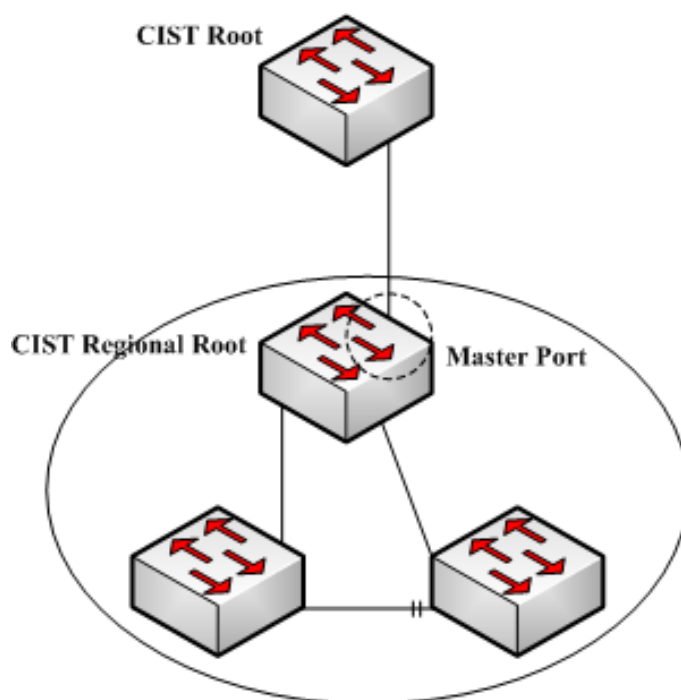
Figure 2.6 Master port
