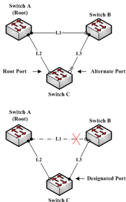
Figure 1.4 Backbone Fast
