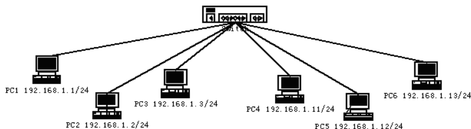
Figure 9 SuperVLAN
