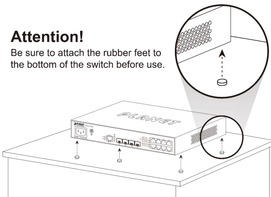
Figure 2-2-1 Place the Managed Switch on the desktop
