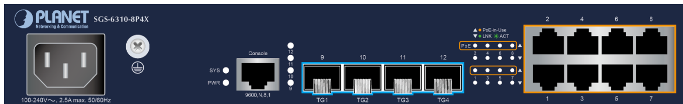
Figure SGS-6310-8P4X front panel
