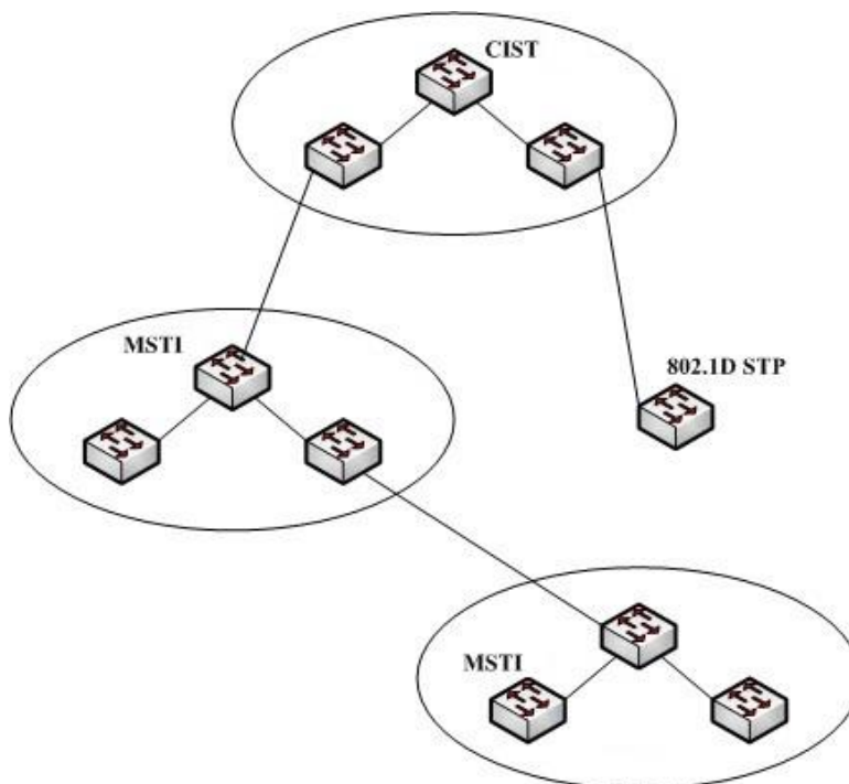
Figure 2.1 MSTP topology
