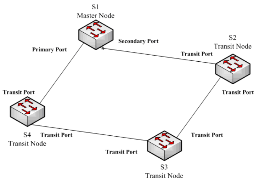
Figure 1.1 EAPS Ethernet ring
